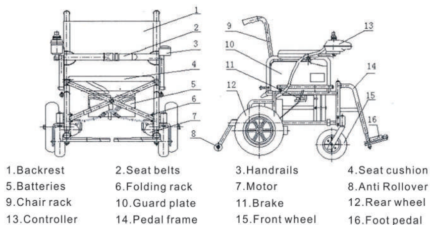
Fig. 1 schematic diagram of electric wheelchair structure
